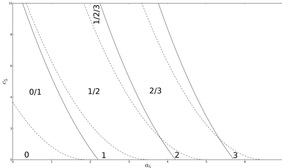
FIGURE 1. Possible values for \alpha_5 as a function of (a_5, c_5) .
