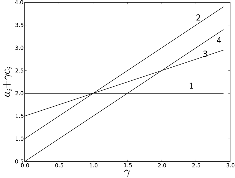
FIGURE 2. Computing \nu_h , h = 1, \dots, 3 .
